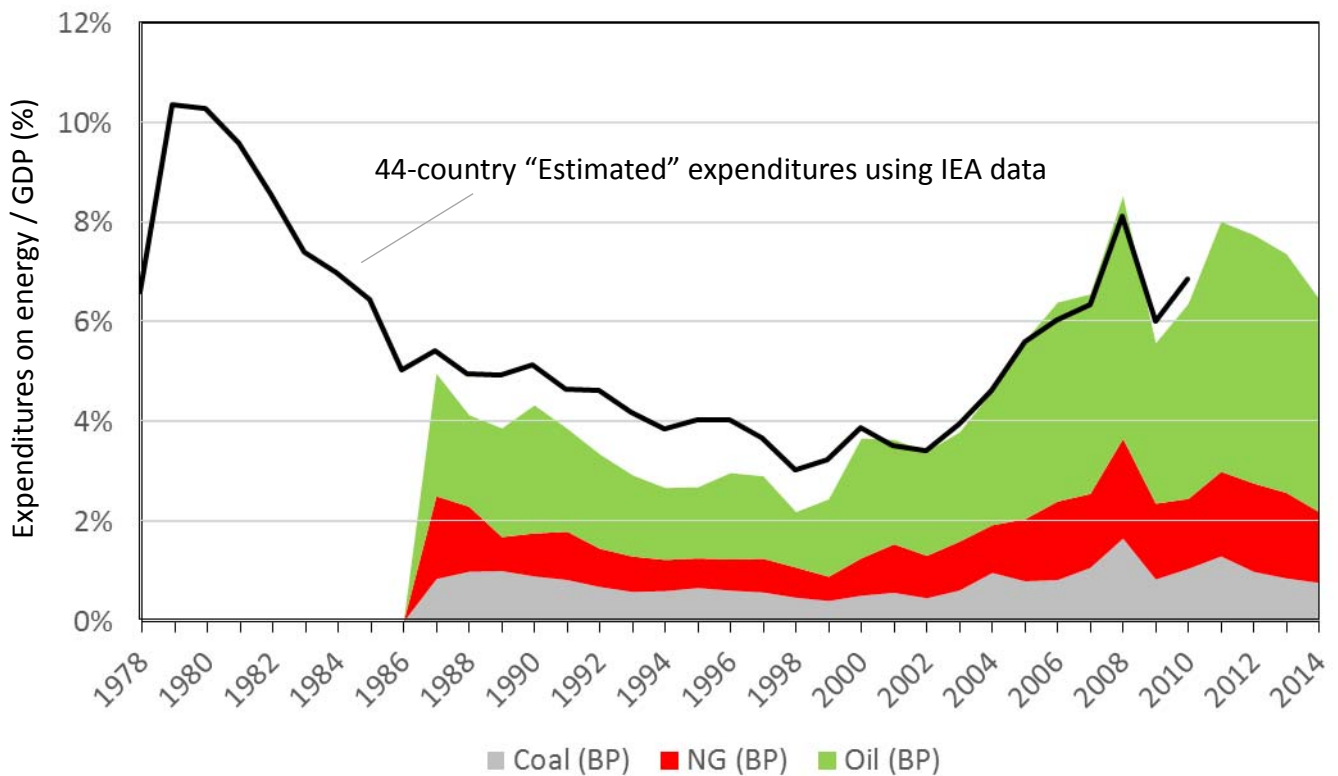
Figure S4. This figure compares two calculations for ‘world’ expenditures on energy divided by GDP, f_{e,GDP} . The black line is our Estimated f_{e,GDP} calculated using the IEA data for the 44-country aggregate. The stacked chart for oil, natural gas, and coal use data from the BP Statistical Review of World Energy and divide by the world GDP (in nominal USD) as provided by the World Bank. Assumed prices for the BP calculations are: nominal crude oil price ($/BBL) from worksheet ‘Oil - Crude prices since 1861’; German import natural gas price ($/MMBtu) from worksheet ‘Gas - Prices ’; and for coal we used the Northwest Europe marker price ($/tonne). Assumed energy consumption for BP calculations are: Total World oil consumption (BBL/yr) from worksheet ‘Oil Consumption - Barrels’; Total World natural gas consumption (Bcf/day) from worksheet ‘Gas Consumption - Bcf’ converted to trillion Btu per using BP’s conversion of 1.01133308326587 TBtu per 1 Bcf; and Total World coal consumption is from worksheet ‘Coal Consumption - Mtoe’ where we use an energy density conversion (Mtoe/million tonnes) as calculated from BP production data from sheets ‘Coal Production - Tonnes’ and ‘Coal Production - Mtoe’.
